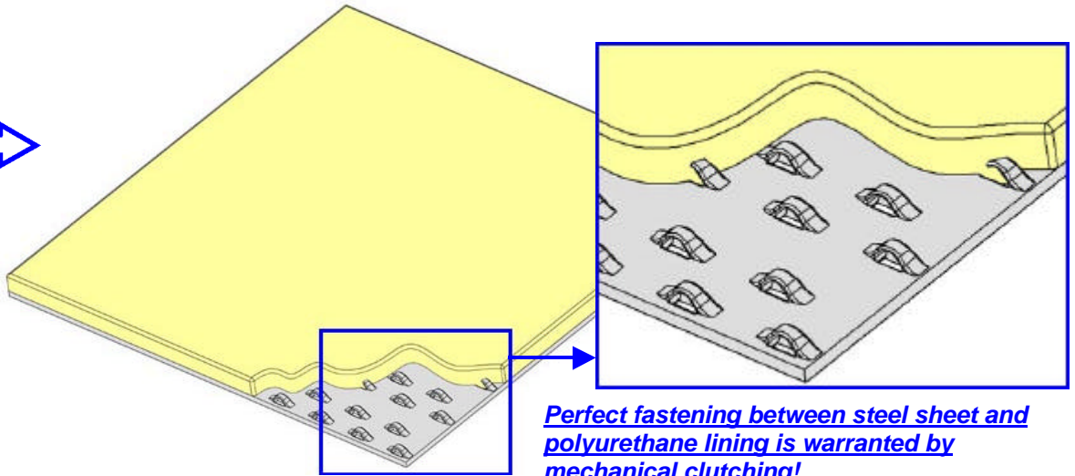
Steel backed polyurethane plates
